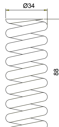
(5) Muelle interior
